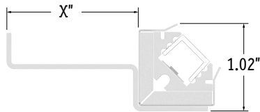
Assembled End View
