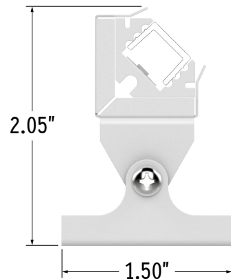
Assembled End View
