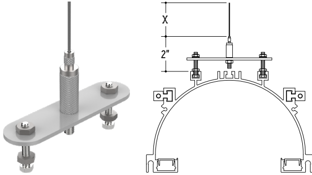
Aircraft Cable Assembly (ALS500T-DBR-AC-6')
