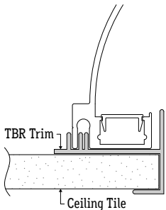
T-Bar Return Ceiling Trim (ALS500T-DBR-TBR)
