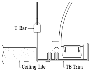
T-Bar Ceiling Trim (ALS500T-DBR-TB)
