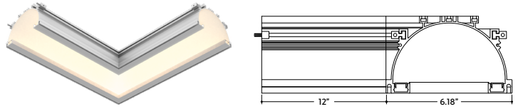
90° Illuminated Corner (ALS500T-DBR-RGBW-90D-X) X = Specify Product Code
