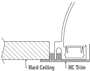
Hard Ceiling Trim (ALS500T-DBR-HC)
