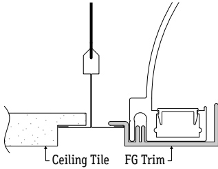
Flange Ceiling Trim (ALS500T-DBR-FG)
