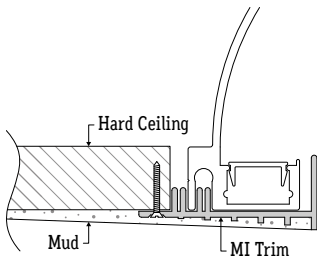
Mud-In Ceiling Trim (ALS500T-DBR-MI)
