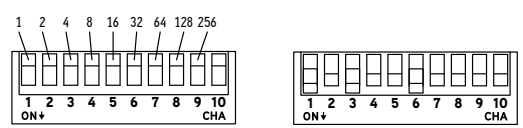
DIP switch value for each switch. Switch 10 has no value (0).
